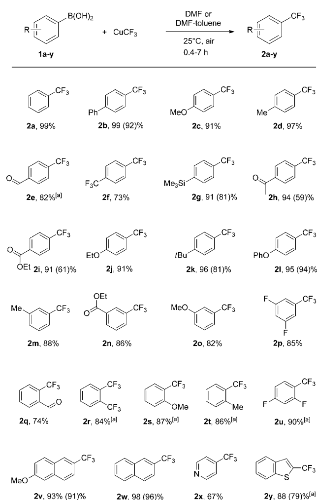
Scheme 3. Trifluoromethylation of aryl boronic acids (0.5–1.0 mmol) with fluoroform-derived CuCF 3 (2 equiv) in air. See the Supporting Information for details. Yields were determined by 19 F NMR spectroscopy with an internal standard. Yields of isolated products are shown in parentheses. [a] At 0 °C.
